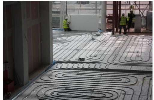
Under-floor heating installation prior to floor screed being laid
